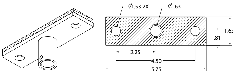
MP-500NPS-TA Tube Adapter
