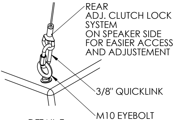
DETAIL E SCALE 1 : 6
