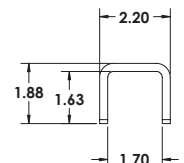
CG-P1377-JBX2 with threaded rod
