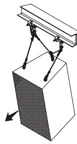
3-Point Suspension
